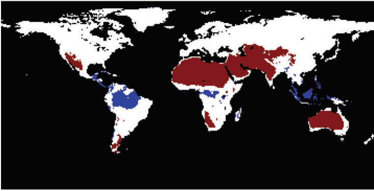
b) Priestley-Taylor (1972) minus Thornthwaite (1948)
