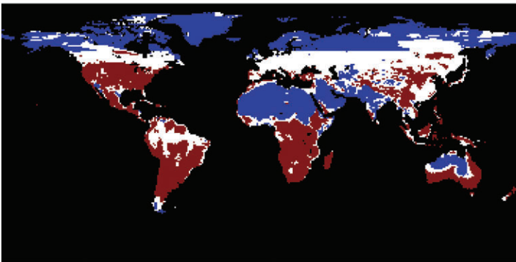
c) Penman-Monteith (1965) minus Thornthwaite (1948)
