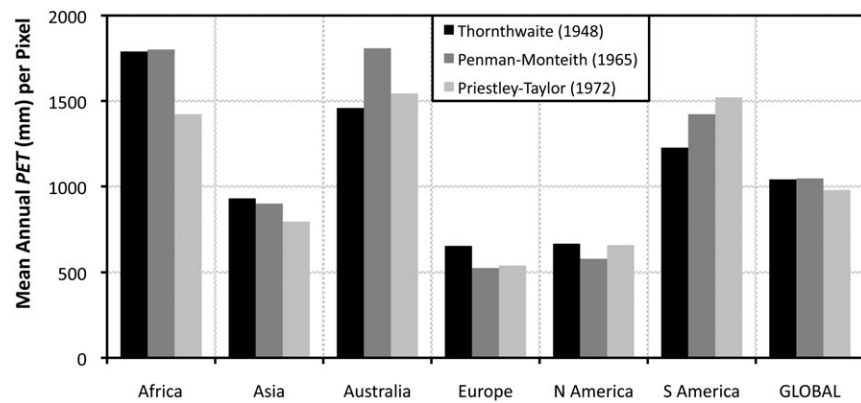
Figure 2 Continental and global mean annual potential evapotranspiration (PET) per pixel ( 0.5^\circ ) estimates for three PET models (Thornthwaite, 1948; Monteith, 1965; Priestley & Taylor, 1972) using ISLSCP-II data for 1990.
